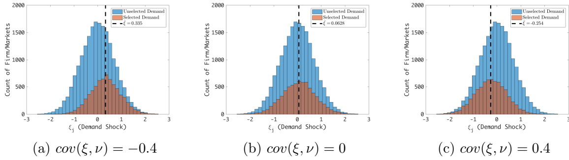
Figure A3: Distribution of Demand Errors ( \xi ) For Different Covariances
