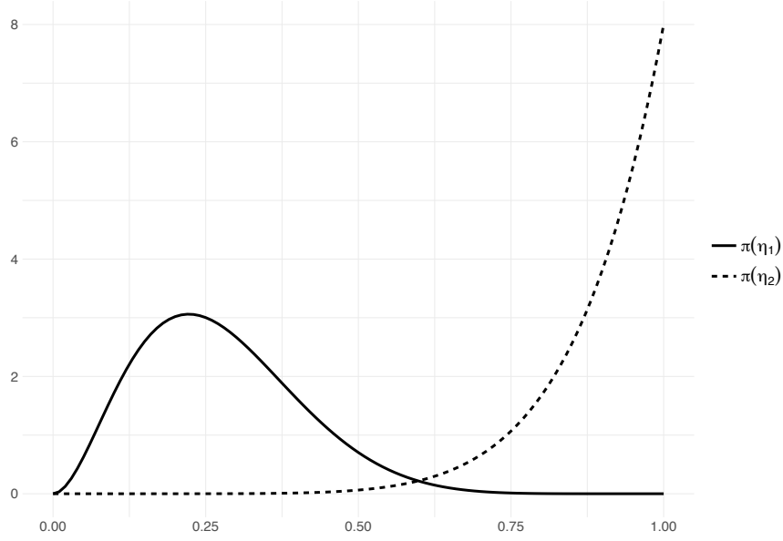
Figure 6: Missing data example: Marginal “curved” priors for \eta_1 (solid line) and \eta_2 (dashed line).
