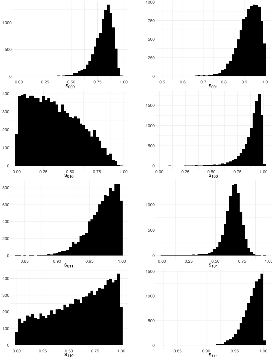
Figure 3: Entry game application: histograms of the SMC draws for selection probabilities s_{000} , s_{001} , s_{010} , s_{100} , s_{011} , s_{101} , s_{110} , and s_{111} for the full model .
