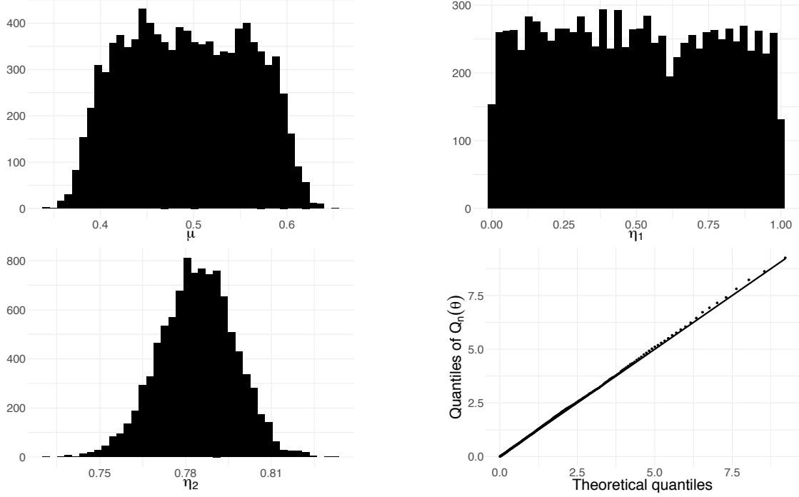
Figure 1: Missing data example: histograms of the SMC draws for \mu (top left), \eta_1 (top right), and \eta_2 (bottom left) and Q-Q plot of Q_n(\theta) computed from the draws against \chi^2_2 quantiles (bottom right) for a sample of size n = 1000 with \eta_2 = 0.8 . The identified sets for \mu and \eta_1 are [0.4, 0.6] and [0, 1] , respectively.
